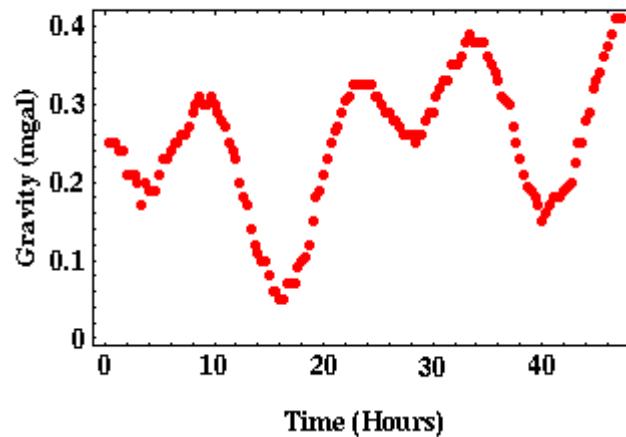
Variation in Gravity, Tulsa Oklahoma, 12/10 - 12/12 1939
