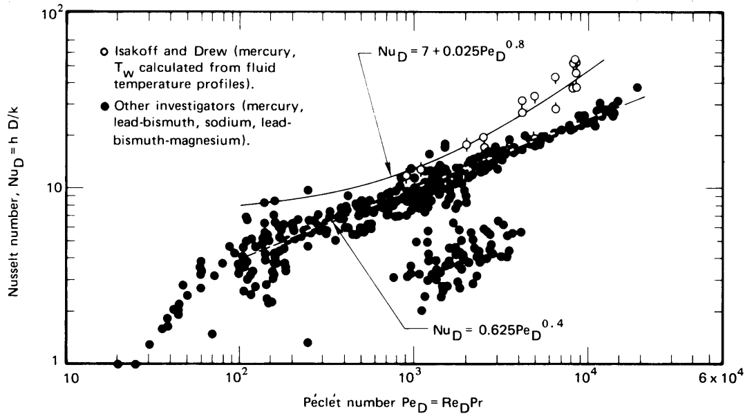
Figure 7.8 Comparison of measured and predicted Nusselt numbers for liquid metals heated in long tubes with uniform wall heat flux, q_w . (See Lubarsky and Kaufman [7.20] for details and data source references.)
