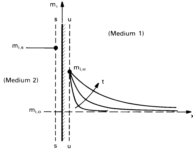
Figure 11.13 Mass diffusion into a semi-infinite stationary medium.
