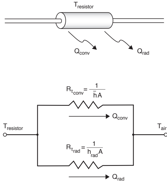
Figure 2.17 An electrical resistor cooled by convection and radiation.
