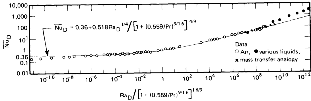
Figure 8.6 The data of many investigators for heat transfer from isothermal horizontal cylinders during natural convection, as correlated by Churchill and Chu [8.10].
