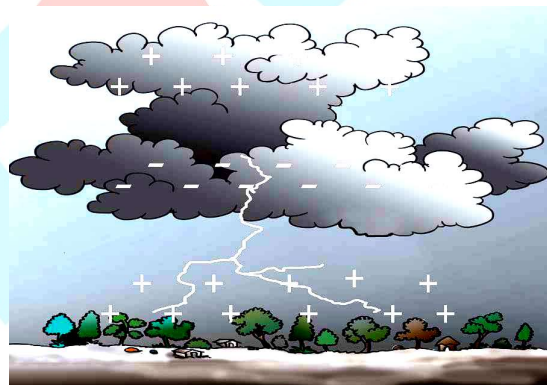
Fig. : Accumulation of charges leading to lightning
