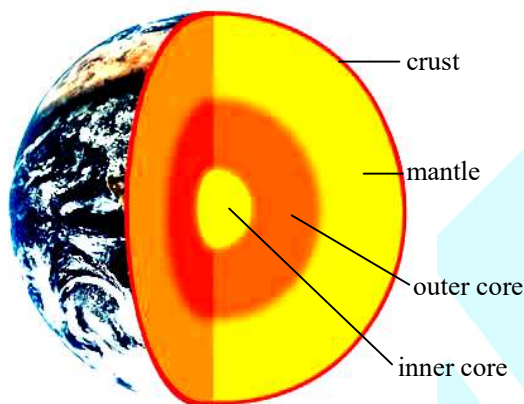
Fig. : Structure of the earth
