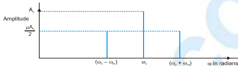
FIGURE-9: A plot of amplitude versus frequency for an amplitude modulated signal
