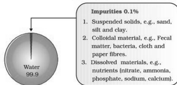
Fig: Composition of waste water
