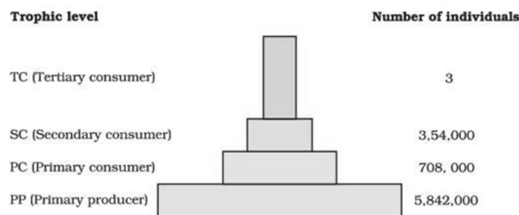
Fig. : Pyramid of numbers in a grassland ecosystem. (For example, only three top-carnivores are supported in an ecosystem based on production of nearly 6 millions plants)
