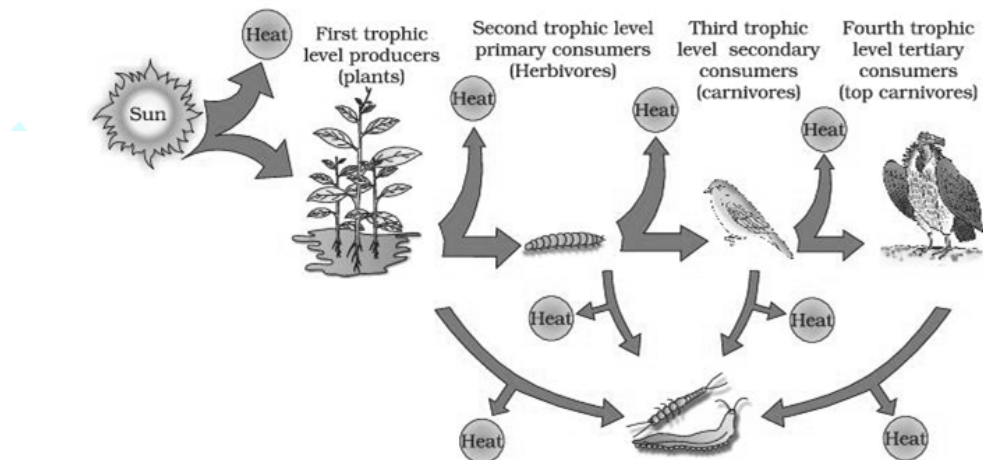
Fig. : Energy flow through different trophic levels
