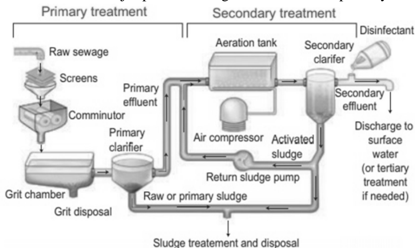
Fig: Sewage treatment plant process flow diagram
