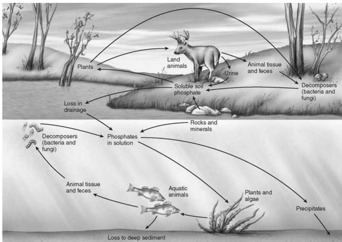
Fig. The phosphorus cycle.
