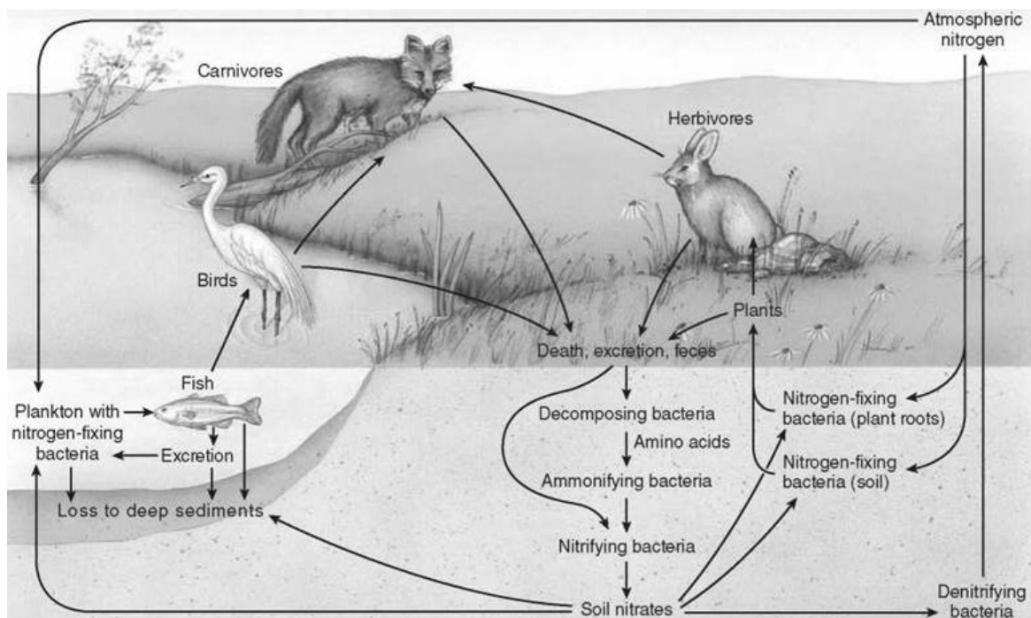
Fig. The nitrogen cycle.
