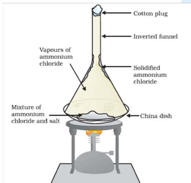
Separation of ammonium chloride and salt by sublimation
