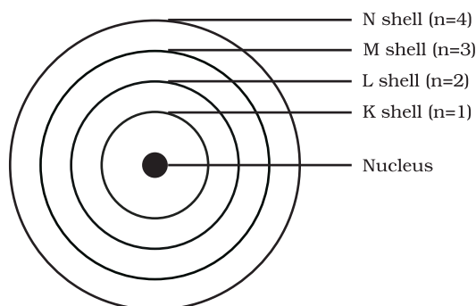
Fig. 4.11: A few energy levels in an atom
