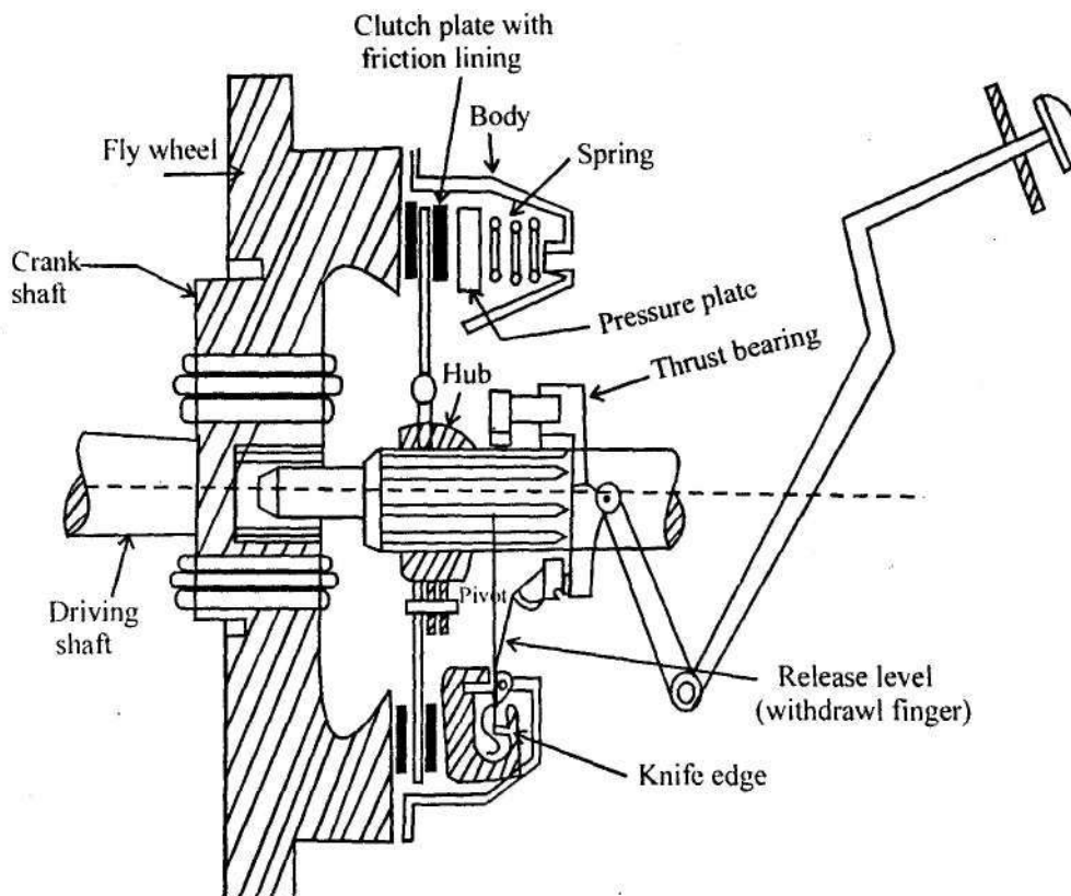
Fig. Single Plate Clutch
